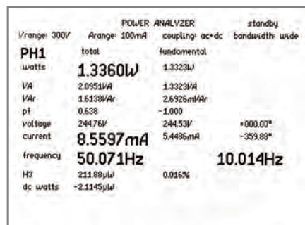
1:5 duty cycle standby power measurement cycle
