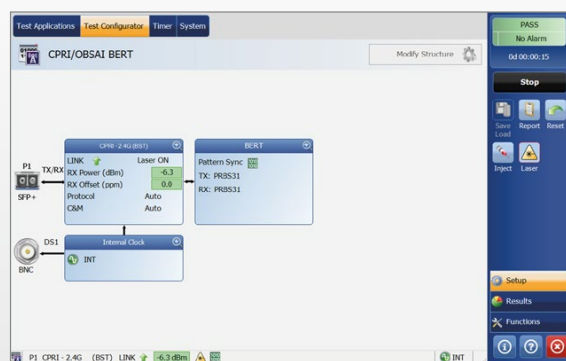
Framed CPRI BER Test
