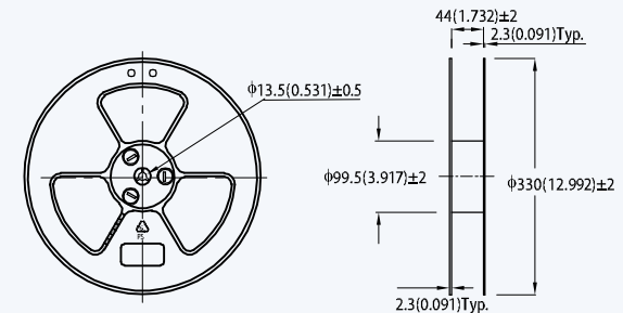
13" (for 44mm width tape)
