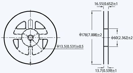
7" (for 12mm width tape)
