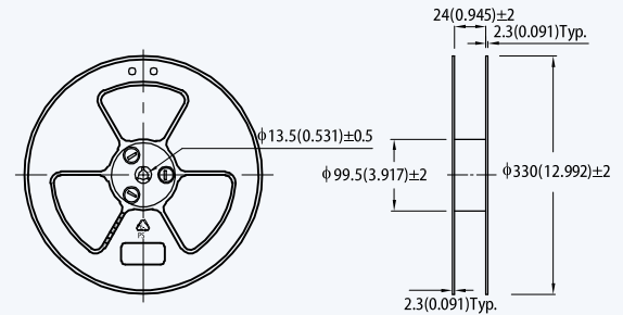
13" (for 24mm width tape)
