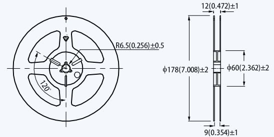
7" (for 8mm width tape) (white)
