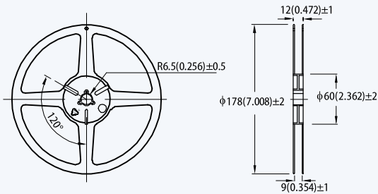
7" (for 8mm width tape) (black)
