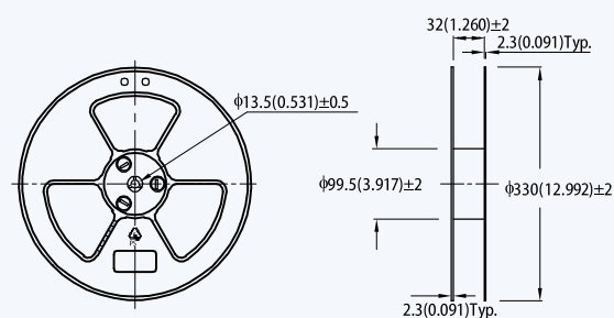
13" (for 32mm width tape)
