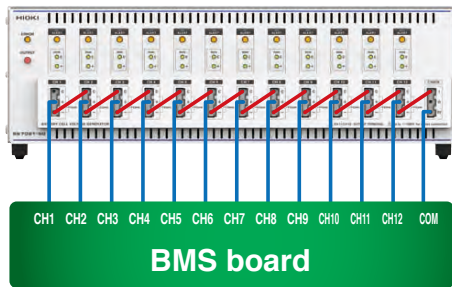
12 channel connection example
