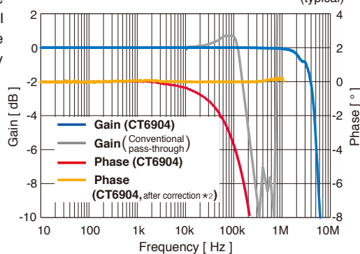
AC/DC CURRENT SENSOR CT6904 frequency characteristics (typical)
