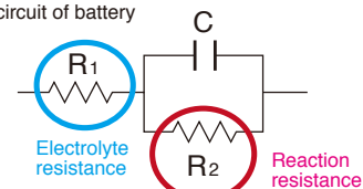
Equivalent circuit of battery
