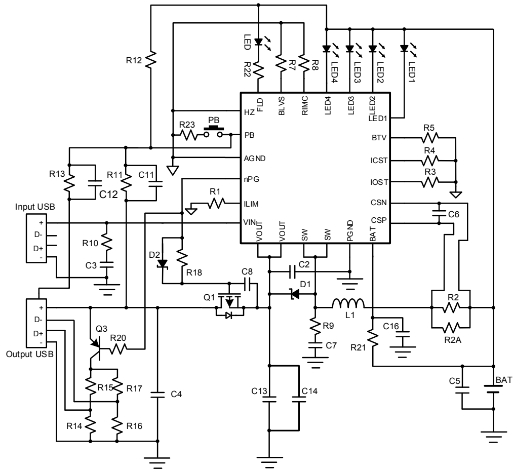
Figure 22. ACT2802B typical application circuit
