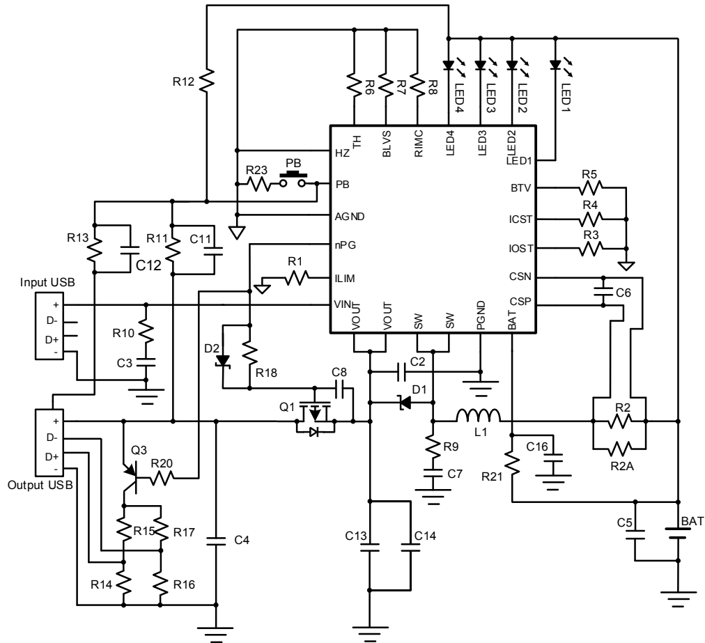
Figure 21. ACT2802 typical application circuit
