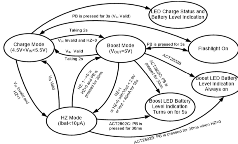
Figure 2: ACT2802B System Operation Flow Chart
