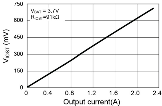
Figure 14. V IOST VS. output current
