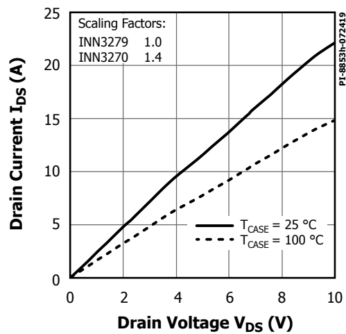
Figure 35. Output Characteristics.
