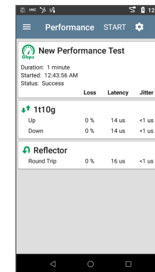
Performance test with up to 8 streams and 8 end points
