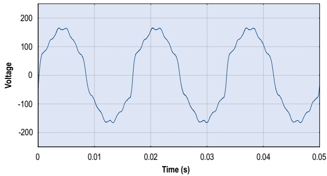
Figure 2 - Simulating Area EPS Voltage Harmonics
