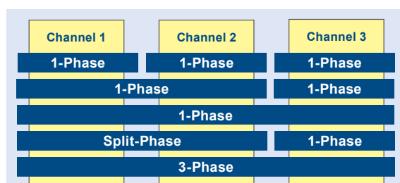
Figure 1 - 3 channels with multiple configuration possibilities.
