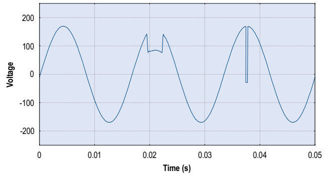
Figure 3 - Simulating Sub-cycle Transients
