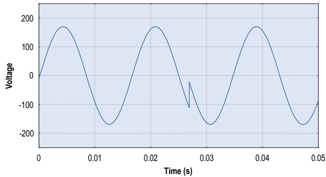
Figure 4 - Simulating Phase Jump
