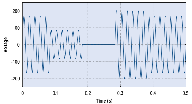
Figure 5 - Simulating abnormal voltages (sags, swells, & drop outs)
