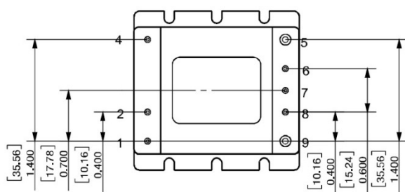
SLOTTED / FLANGED BASEPLATE
