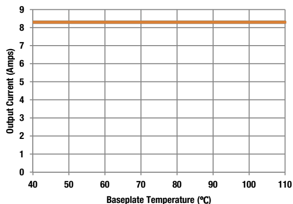
Figure 14 Thermal Derating vs. Baseplate temperature
