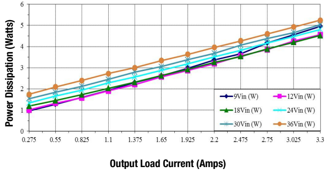
24QS15.50SBM Power Dissipation vs. Line and Load
