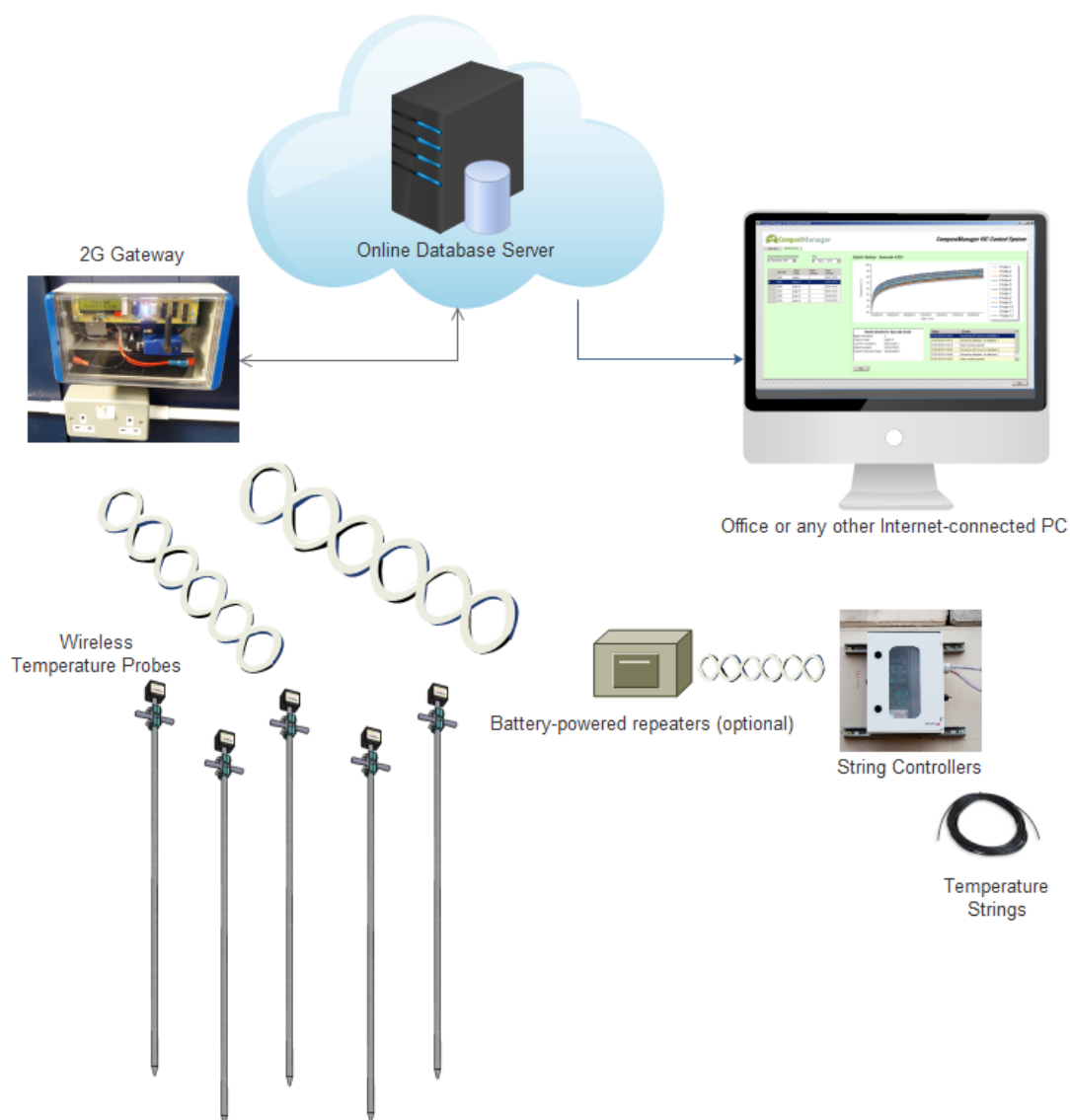
Figure 1. Overview of data transfer for smarTprobes wireless probe system, showing optional string data sensors and signal repeaters
