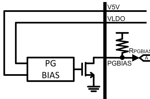
Figure 43. PGBIAS Block
