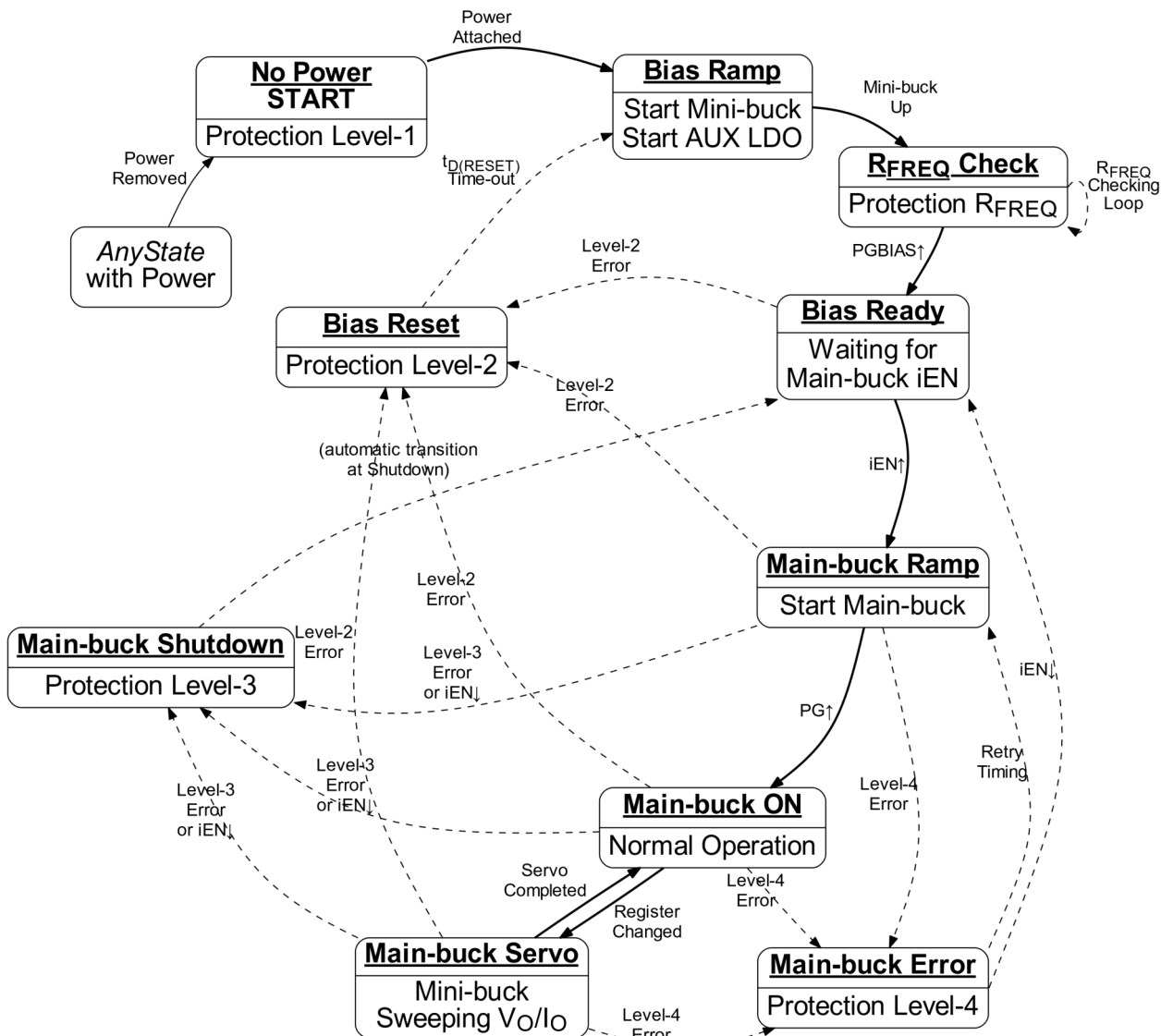
Figure 37. State Diagram
