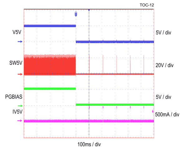
Figure 15. Mini-buck Short Circuit Protection
