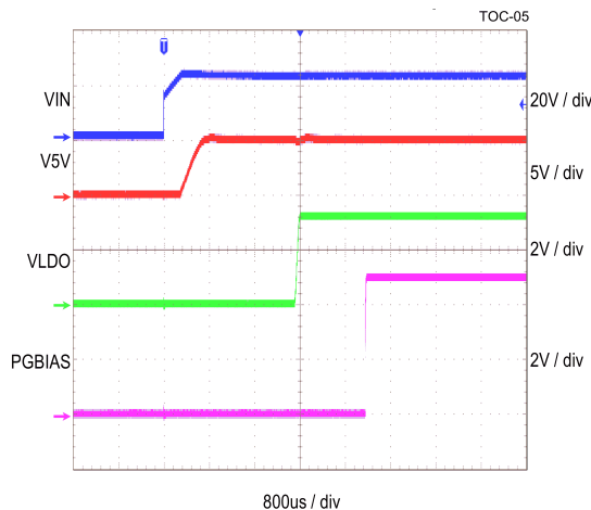
Figure 8. Mini-buck Startup
