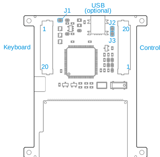
DPP-CTS2432 connections (view from PCB side) See Pin Descriptions
