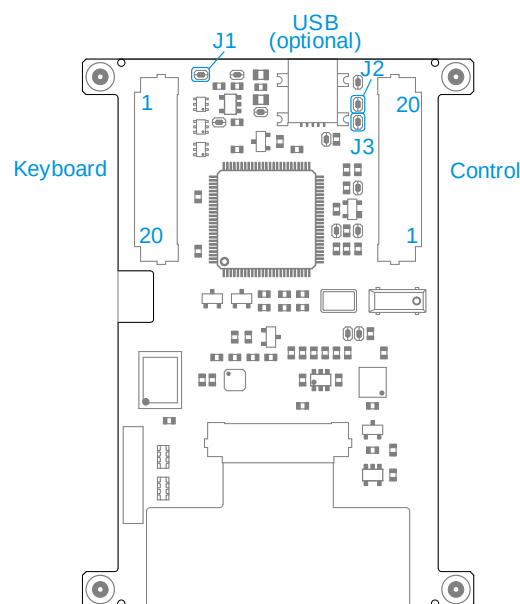
DPP-CTS2440 connections (view from PCB side) See Pin Descriptions
