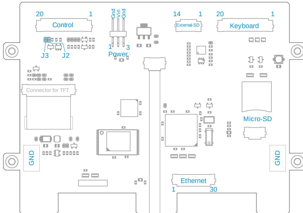
DPP-x57 connections (view from PCB side) See Pin Descriptions
