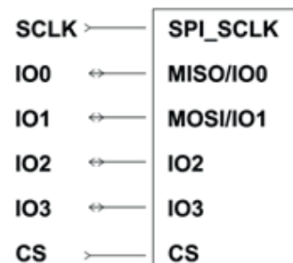
Figure 7. QSPI interface connection
