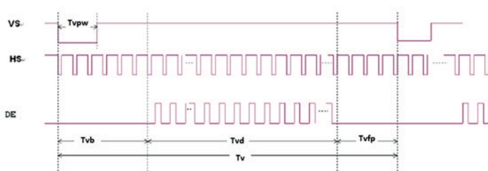
Figure 12. Vertical input timing diagram
