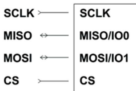
Figure 6. SPI interface connection
