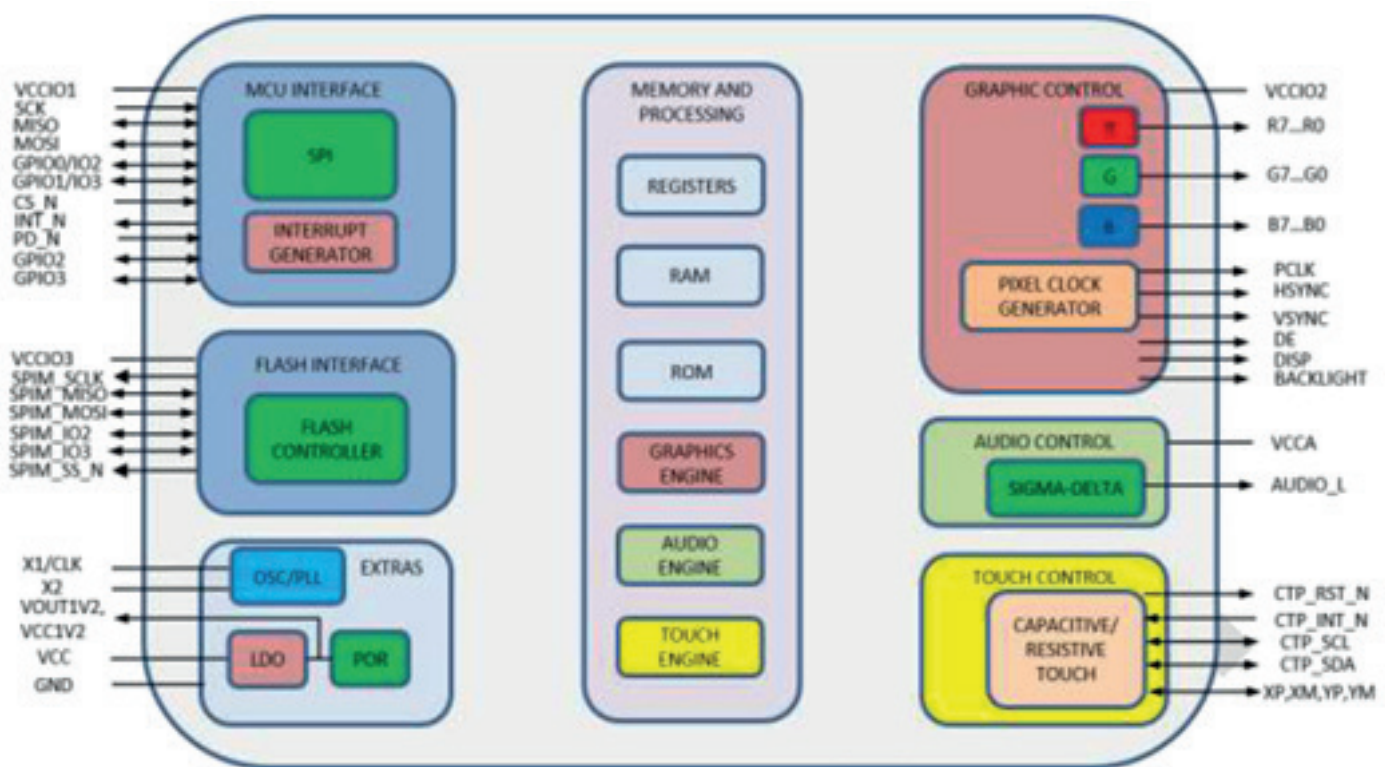
Figure 8. BT8x Block diagram
