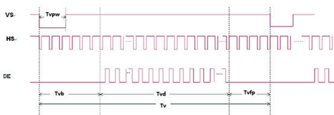
Figure 12. Vertical input timing diagram
