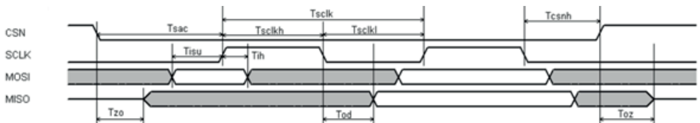
Figure 9. SPI timing diagram
