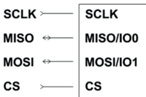
Figure 6. SPI interface connection
