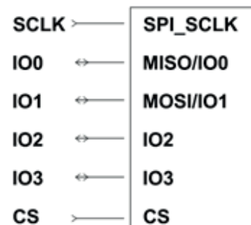
Figure 7. QSPI interface connection
