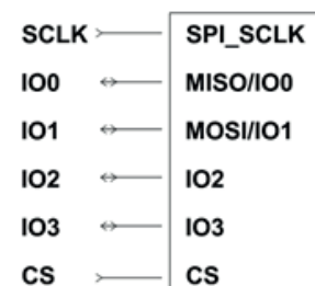
Figure 7. QSPI interface connection
