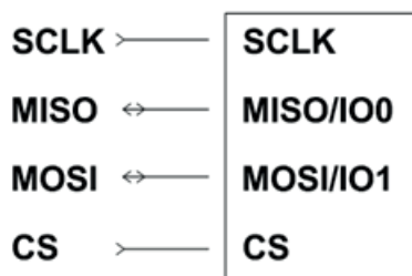
Figure 6. SPI interface connection
