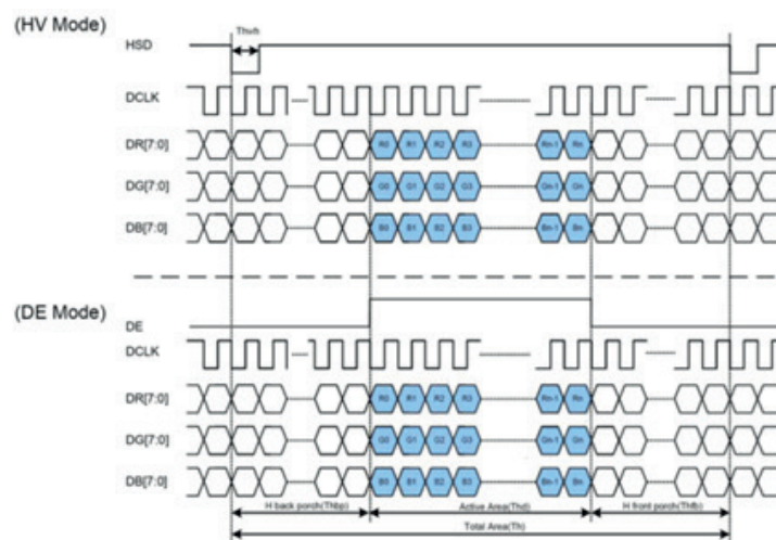
Figure 11. Clock and data input time diagram
