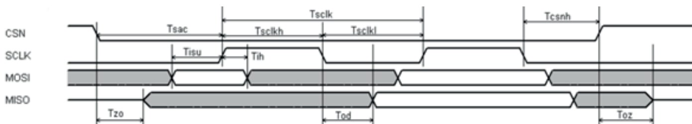
Figure 9. SPI timing diagram
