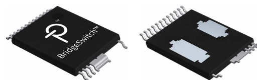
Figure 2. InSOP-24C Package (Top and Bottom Sides).
