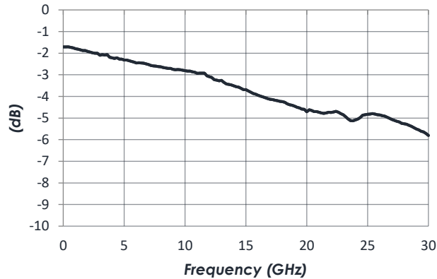
Insertion Loss
