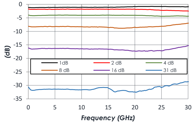
Normalized Major Attenuation States
