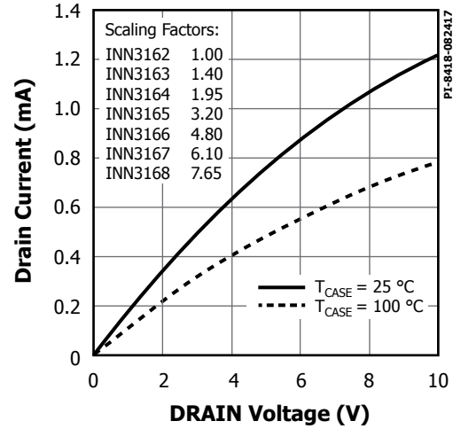
Figure 22. Output Characteristics.
