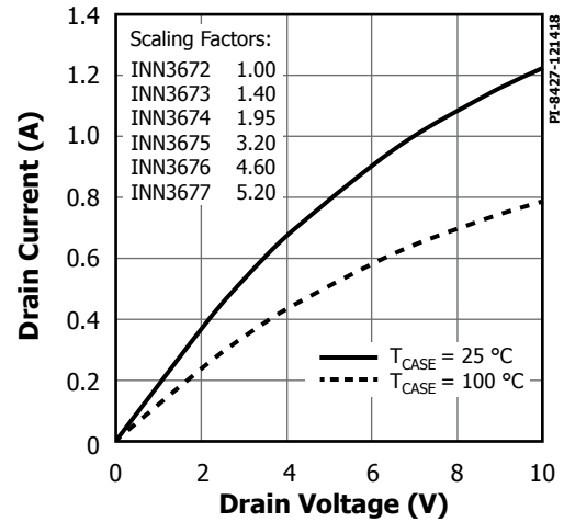
Figure 25. Output Characteristics.
