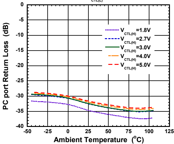
Return Loss vs Temperature
