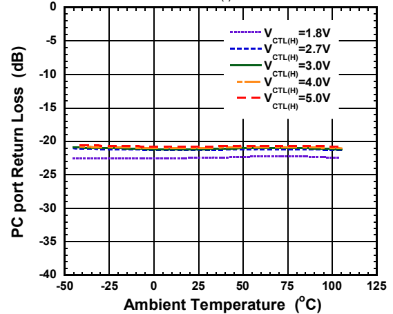
Return Loss vs Temperature
