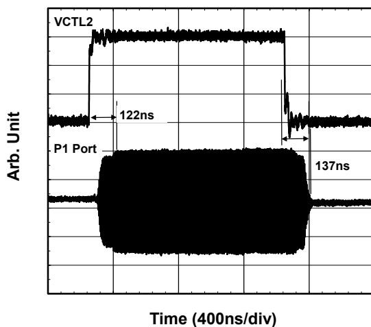
Switching Time
