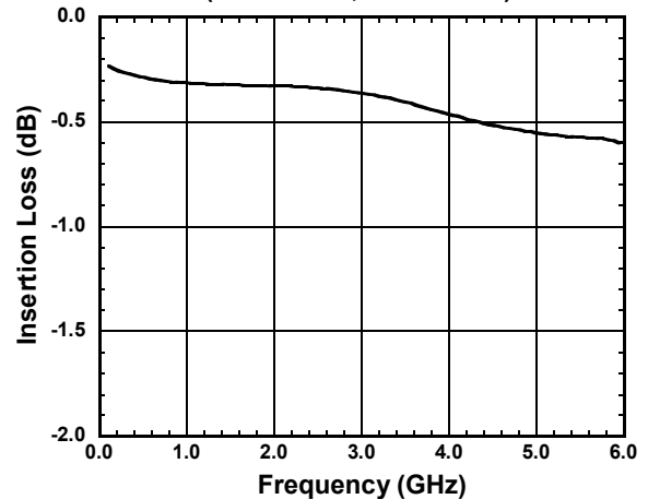
PC-P2 Insertion Loss vs. Frequency ( VCTL1=3V, VCTL2=0V )
