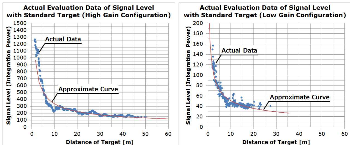
Fig. 9 Actual Evaluation Data of Signal Level
