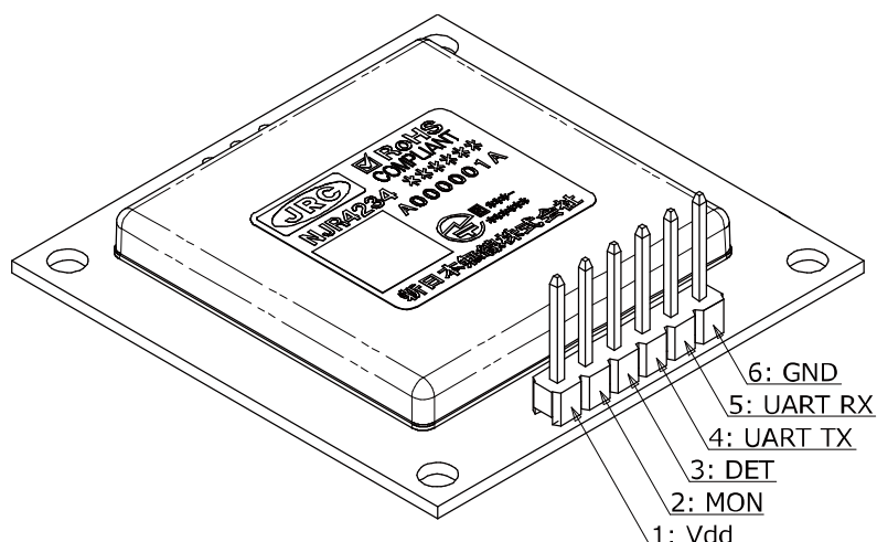
Fig. 13 Pin Diagram
