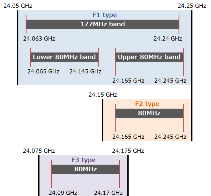
Fig. 12 Frequency Plan
