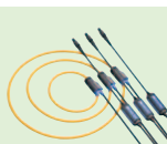
AC FLEXIBLE CURRENT SENSOR CT9667-01/-02/-03 \phi 100/180/254 mm (3.94/7.09/10.00 in)
