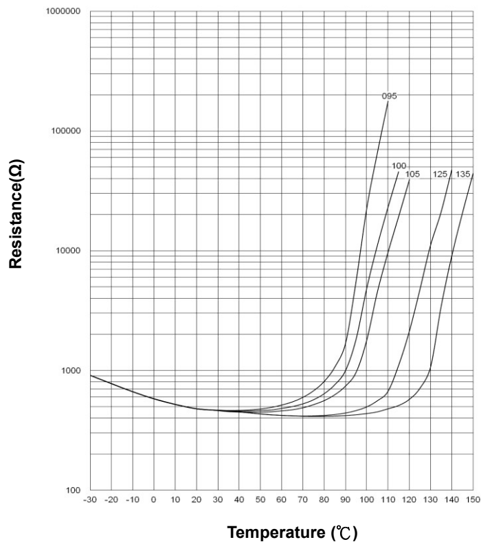
SMD 0805 R25= 470 \Omega TPM2C471PXXXR
