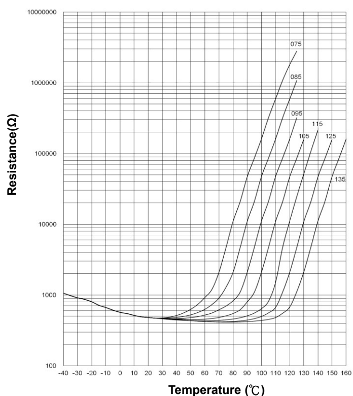
SMD 0603 R25= 470Ω TPM1C471PXXXRT
