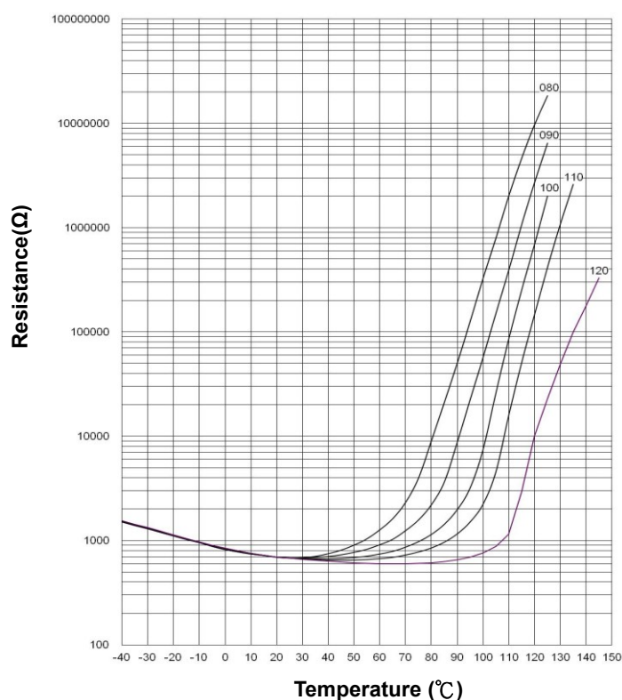
SMD 0805 R25= 680 \Omega TPM2C681PXXXR
