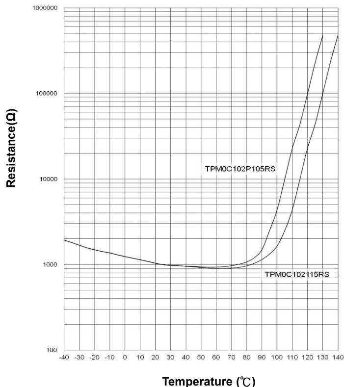
SMD 0402 R25= 1KΩ TPM0C102P105RS & TPM0C102P115RS
