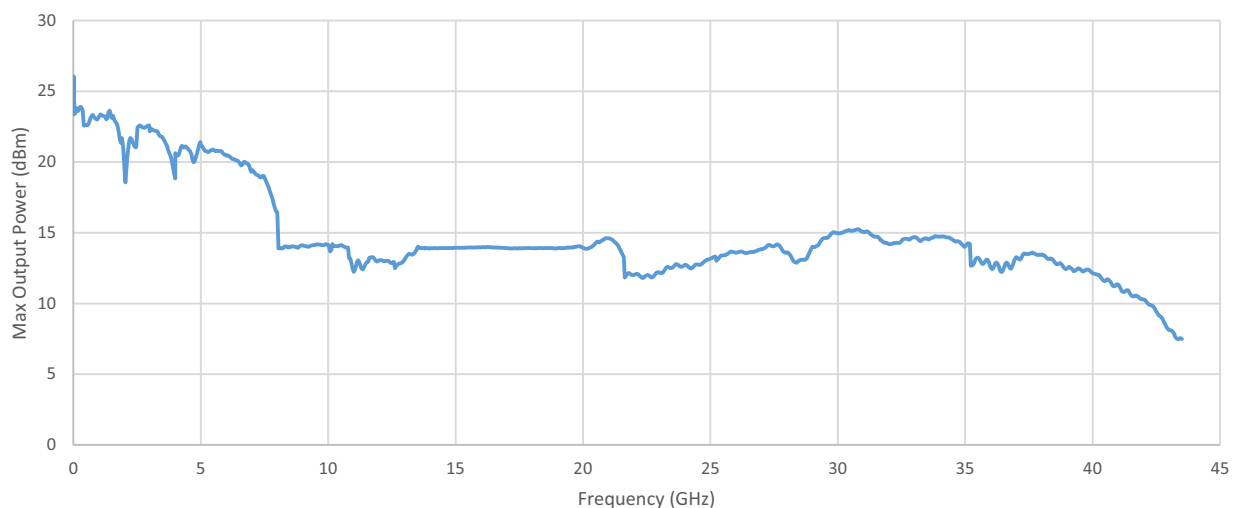
MS46524B Example Maximum Port Power
