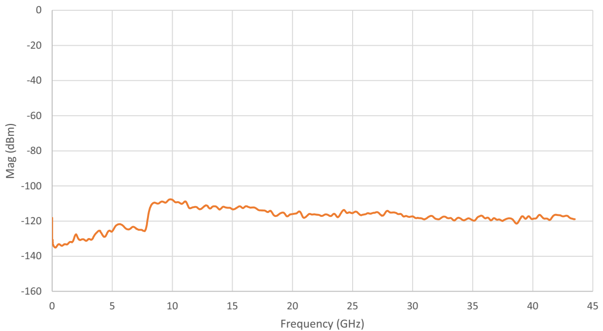
MS46524B Example Noise Floor
