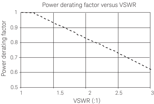
Figure 9. Power derating factor versus VSWR
