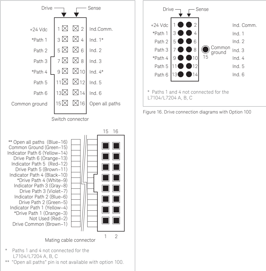
Figure 15. Drive connection diagrams with Option 161
