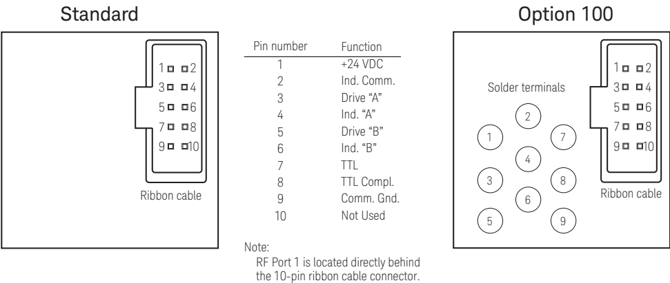
Figure 6. Drive connections
