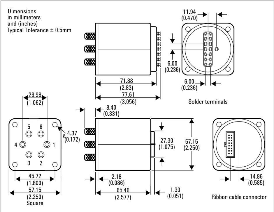
Figure 10. Product outline
