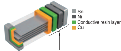
Soft termination (Conventional type)
