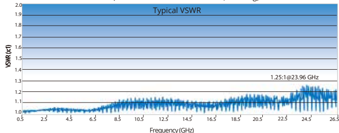
Cable is pulled off center 10° in both directions
