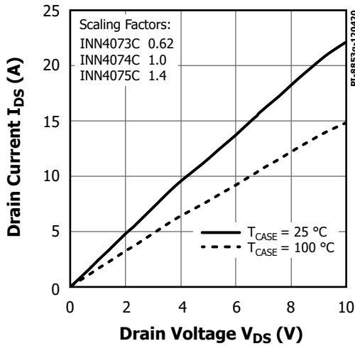
Figure 21. Output Characteristics.
