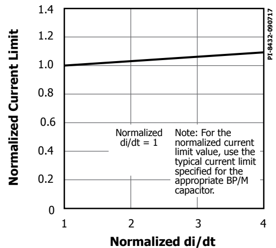
Figure 26. Standard Current Limit vs. di/dt .
