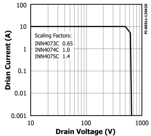
Figure 24. Maximum Allowable Drain Current vs. Drain Voltage.
