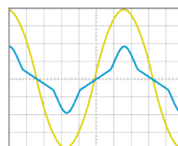
110V, 5A + 22 ohms Test Waveform
