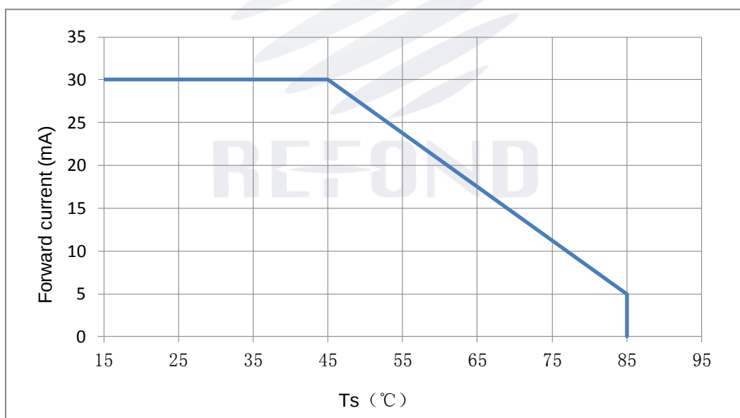
Fig 1-11 Solder Temperature Vs Forward Current 管脚温度与正向电流特性曲线
