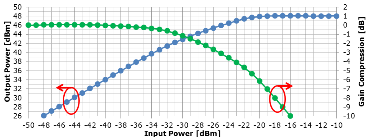
Output Power/Gain Compression vs. Input Power
