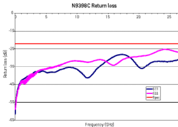
Figure 6. N9398C typical return loss versus frequency
