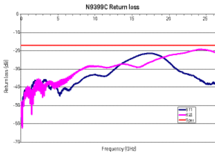
Figure 8. N9399C typical return loss versus frequency
