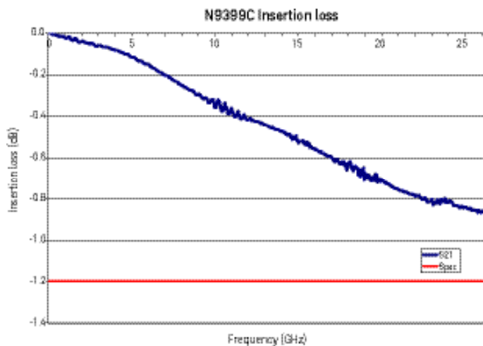
Figure 9. N9399C typical insertion loss versus frequency
