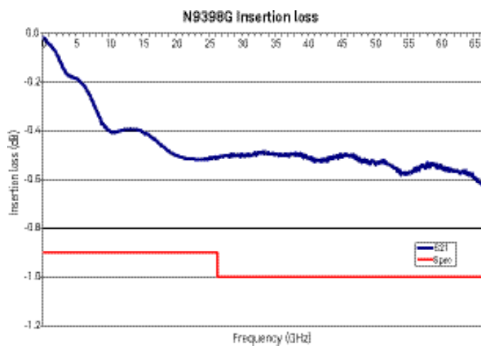
Figure 15. N9398G typical insertion loss versus frequency
