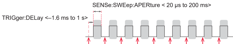
Figure 1. The X-Series power sensor offers real time measurement by measuring every consecutive pulse without dead time.
