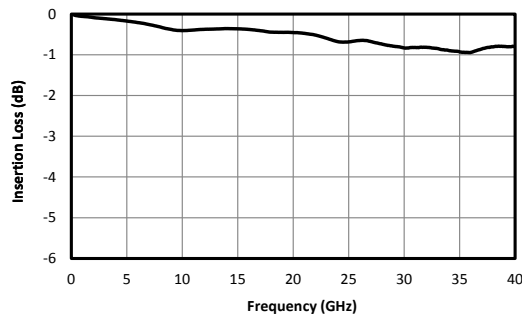
Figure 1. Insertion Loss
