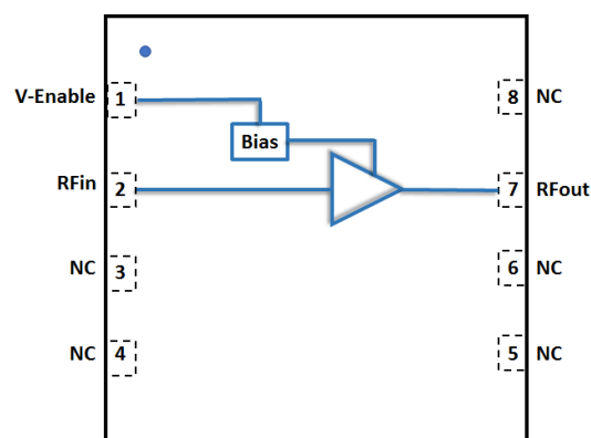
Figure 3.1 Function Block Diagram (Top View)
