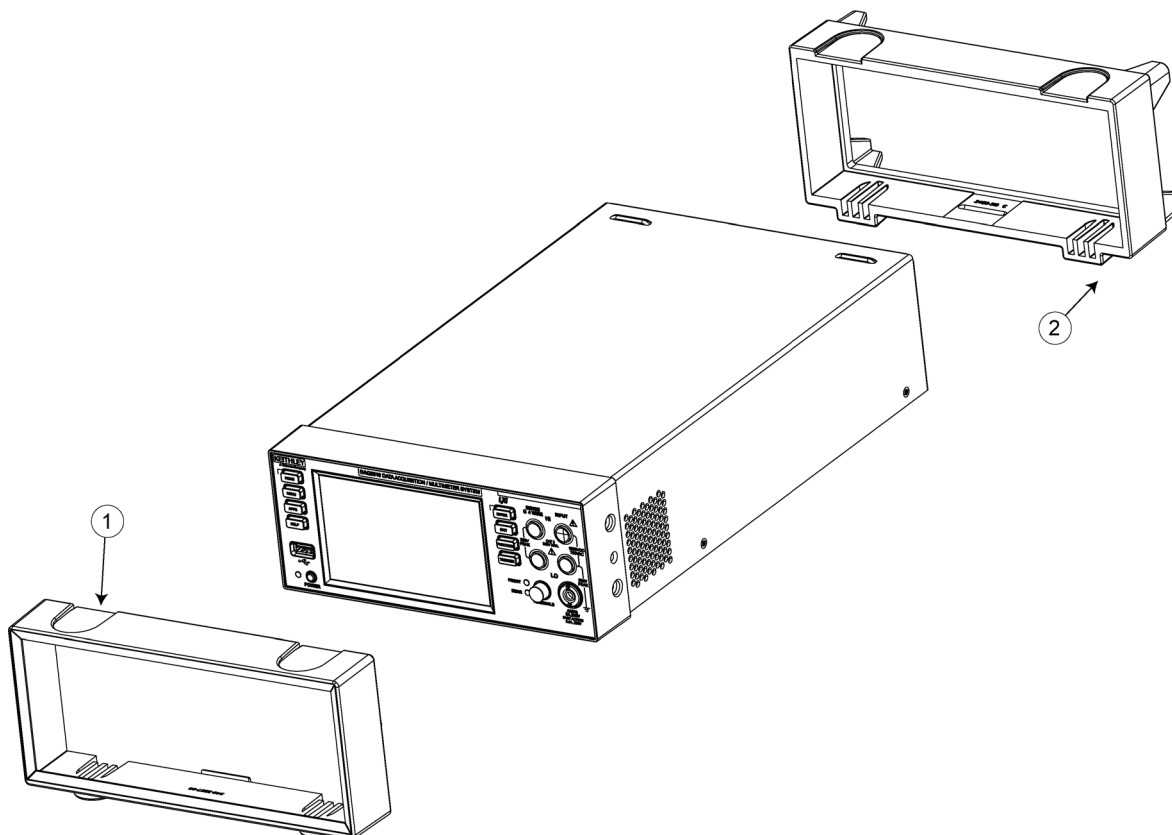
Figure 6: Remove bumpers
