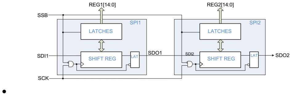
Figure 7: SPI with 2 ICs Daisy-chained
