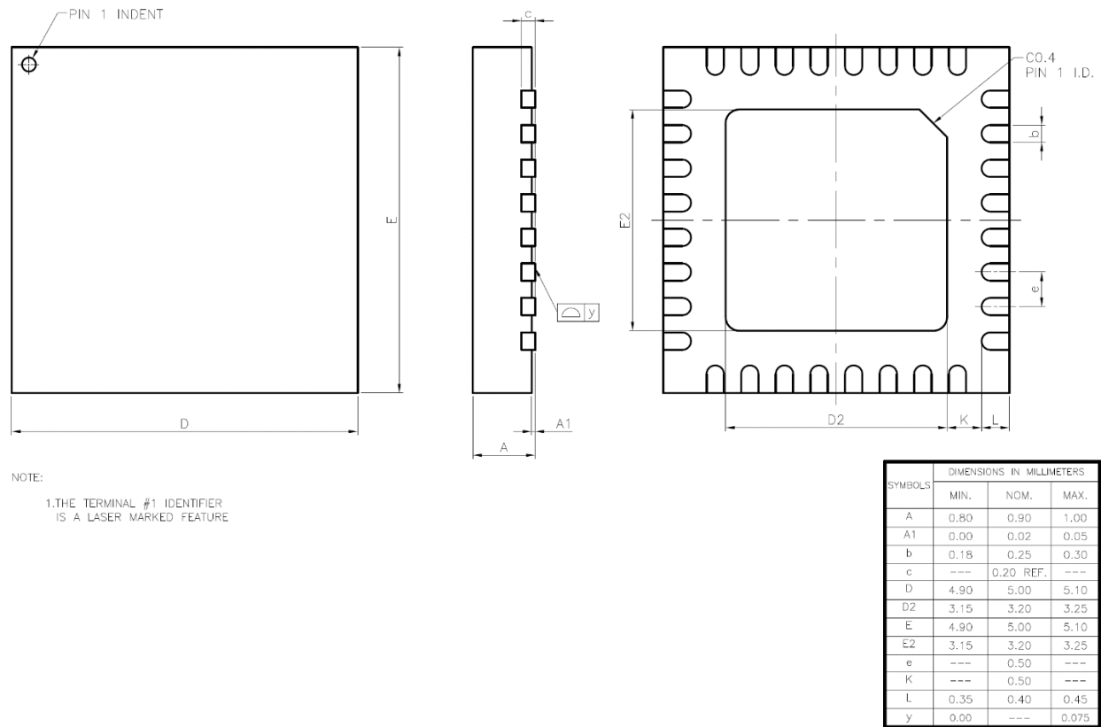
Figure 11 QFN Package Drawing
