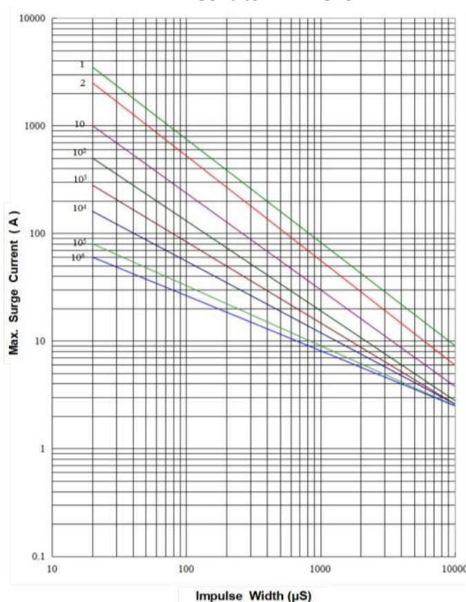
TVB DS820 to TVB DS751
