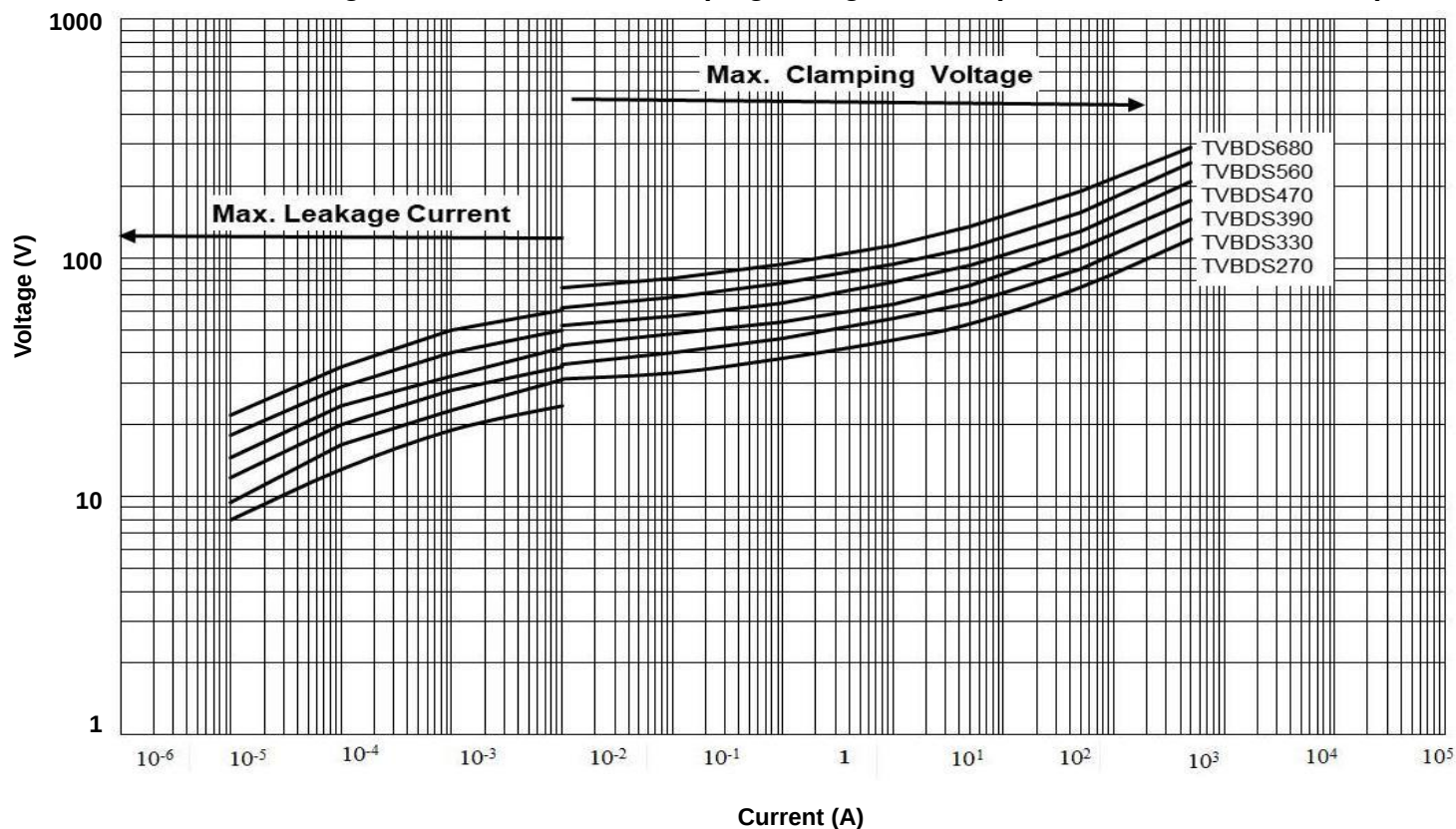
Max. Leakage Current and Max. Clamping Voltage Curves (TVB DS 270 to TVB DS 680)
