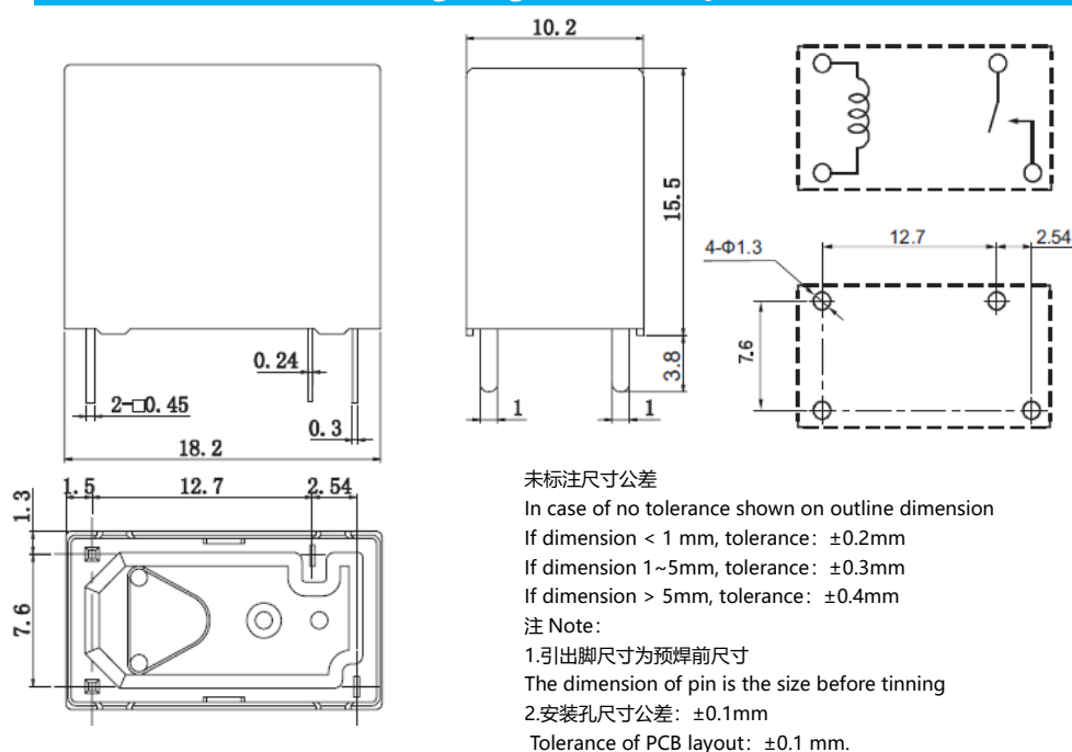
接线图 (底视图) Wiring Diagram (bottom view)
