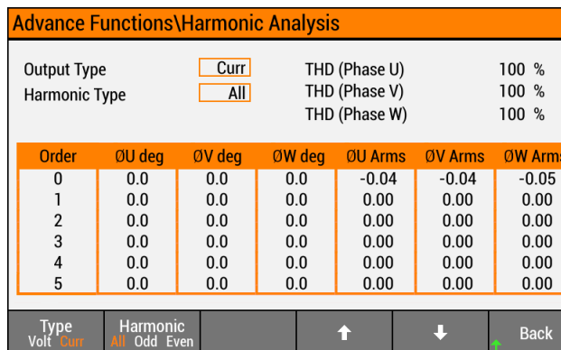
Figure 5. Analyze current or voltage harmonics up to 50 th order
