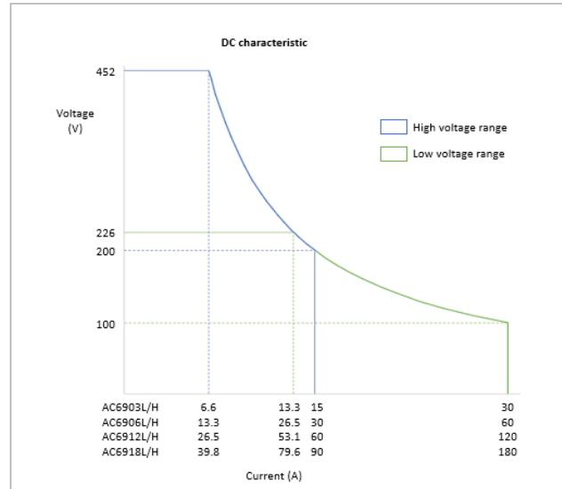
Figure 10. DC characteristic
