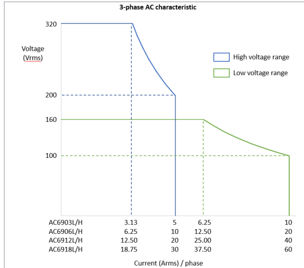
Figure 9. 3-phase AC characteristic
