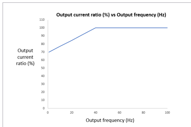
Figure 11. Output current ratio (%) vs Output frequency (Hz)
