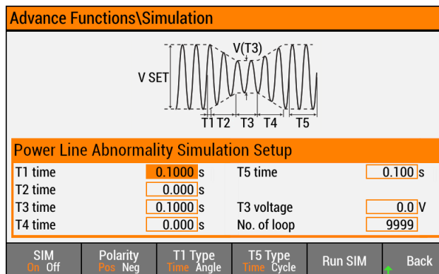
Figure 3. Simulate power outage, surge and sag for environmental testing on your devices
