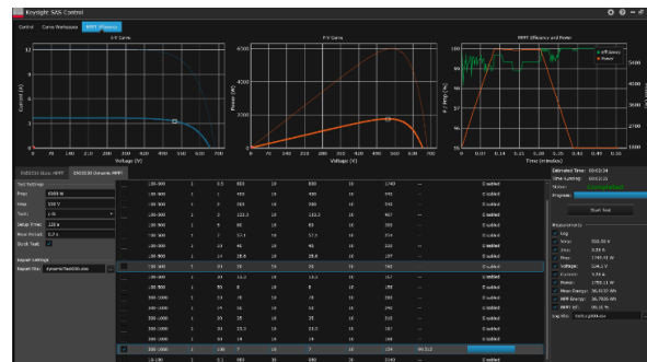
Figure 11. DG9801 performing EN50530 MPPT
