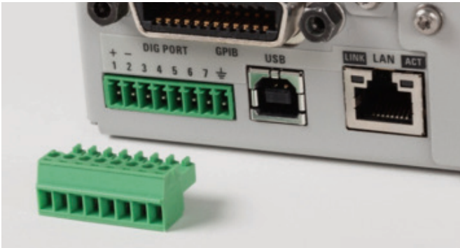
Figure 10. Digital control port on rear panel
