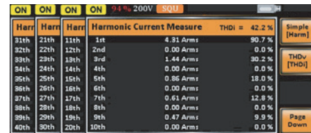
Current Harmonic
