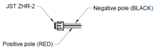
LED connector View
