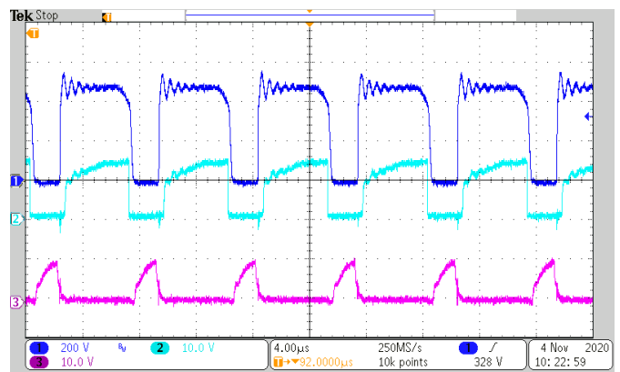
V_{in} = 230Vac/50Hz , 100% Load
